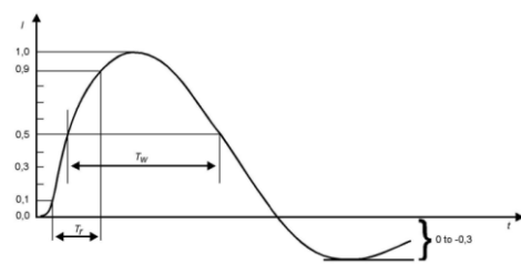
Short-circuit figure
